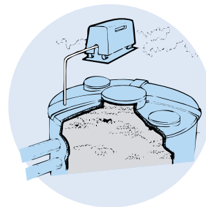
曝气式净化槽
